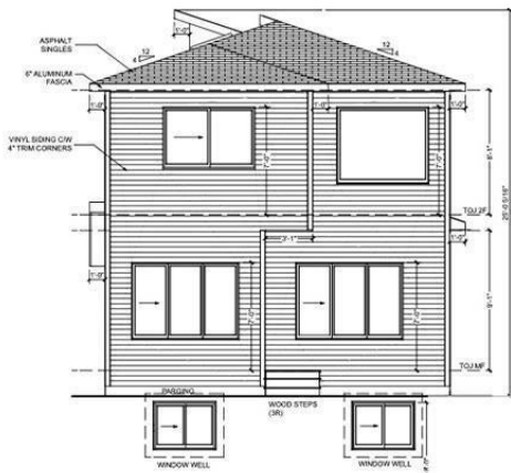
REAR ELEVATION
